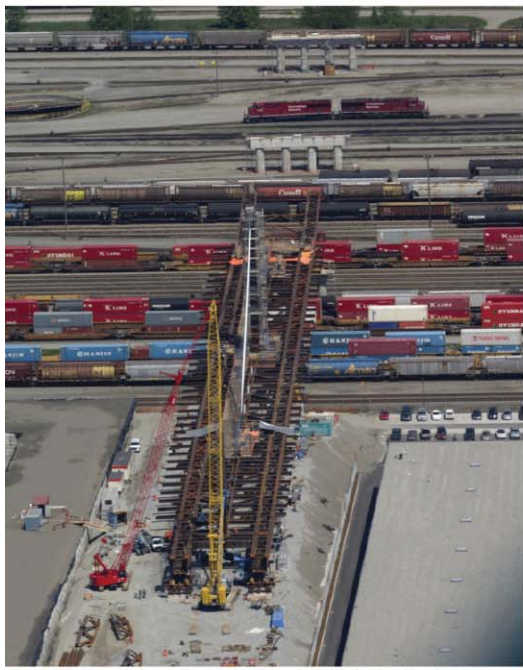
Aerial view of push-launch of CMO deck structure.
